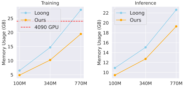
Figure 7: GPU memory usage for training (single A100, batch size 1) and inference (single A100, batch size 16). The dotted line is the GPU memory of NVIDIA 4090 GPU (24GB).
