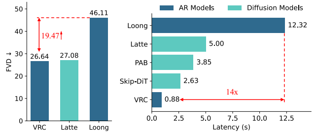
Figure 1: Comparison of FVD and inference time (for 17 frames) across models on a single A100 GPU on FaceForensics (Rössler et al. 2018). VRC (ours) achieves better FVD ( Left ) and faster inference ( Right ) than Loong (our LLM-based baseline (Wang et al. 2024d)) and Latte (Ma et al. 2024).
