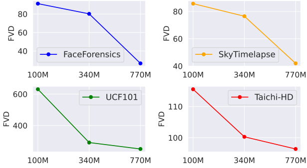
Figure 5: Performance comparison on various class-to-video datasets across different model sizes of our method.
