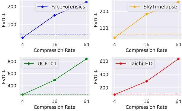
Figure 6: Performance of different compression rates on various datasets. The dotted line is the FVD score of the baseline without any representation compression (Loong*).
